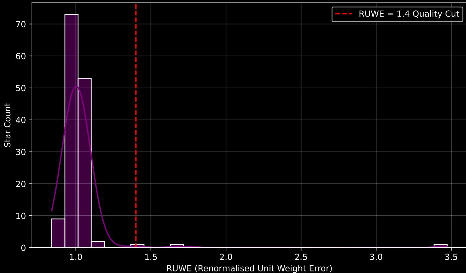
GAPOGEE DR17 Field [SMC8] RUWE Distribution (n= 140)
