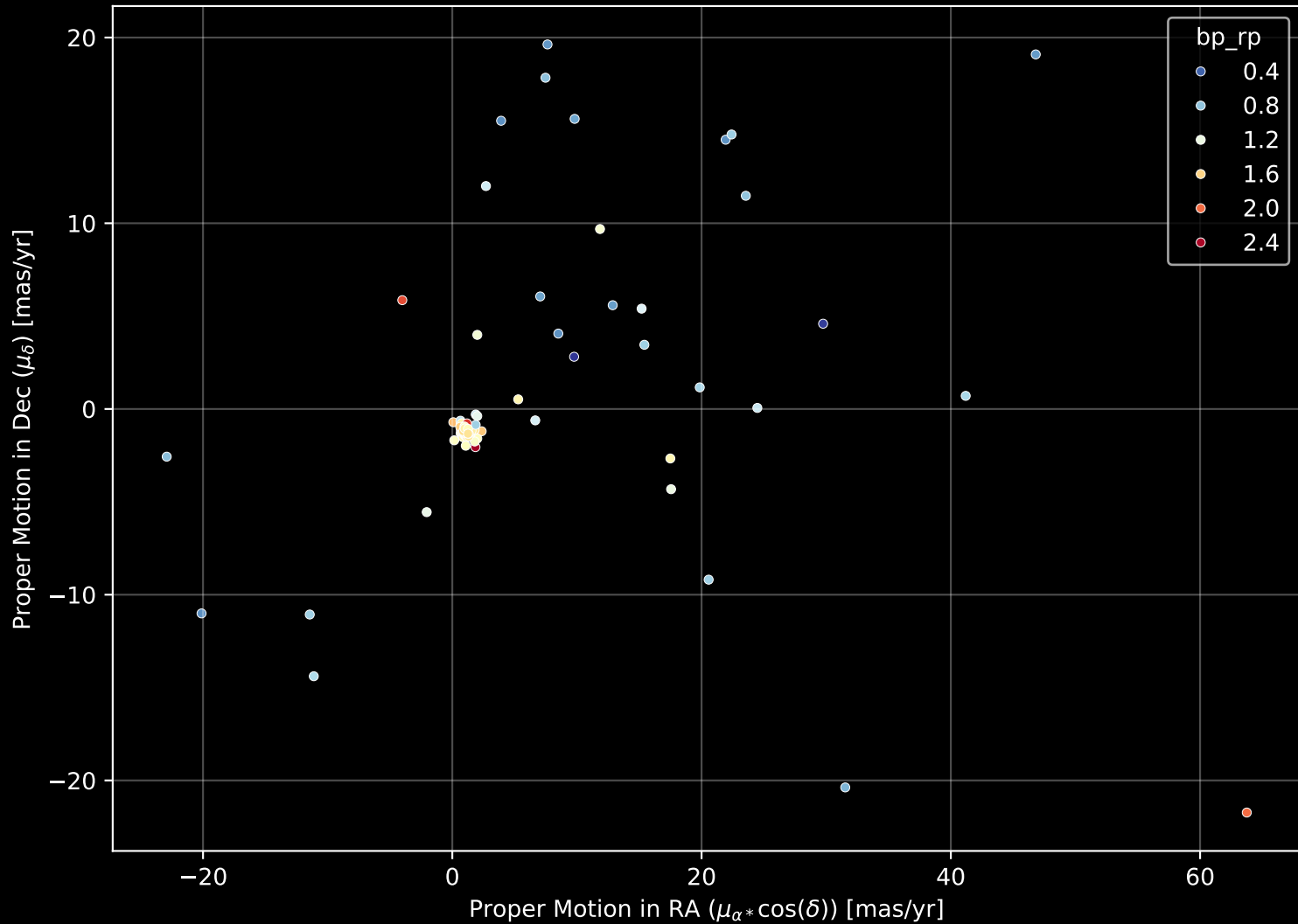
APOGEE DR17 Field: [SMC8] Proper Motion Diagram (n= 142)
