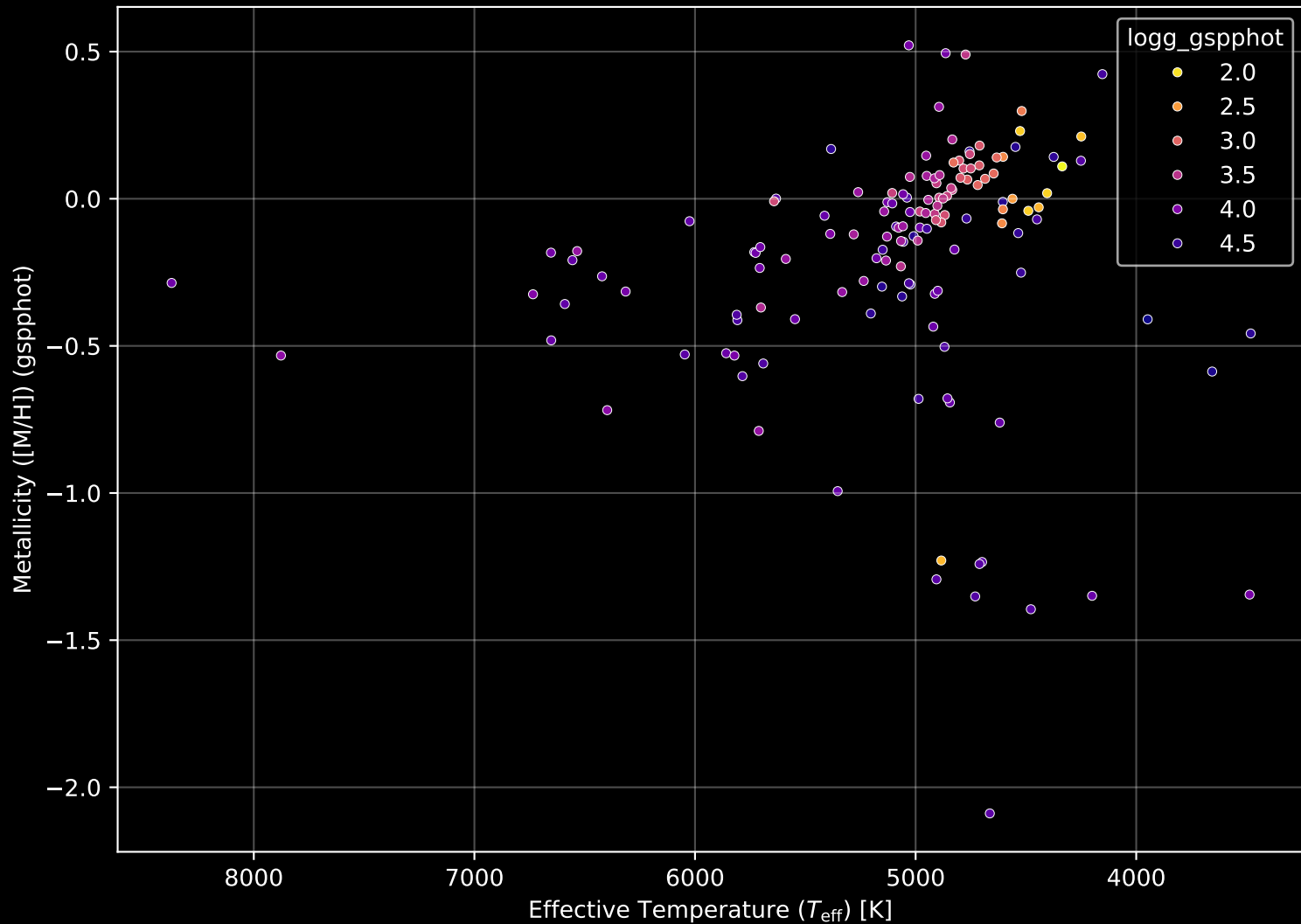
APOGEE DR17 Field: [SMC8] Stellar Population Parameters (n= 142)
