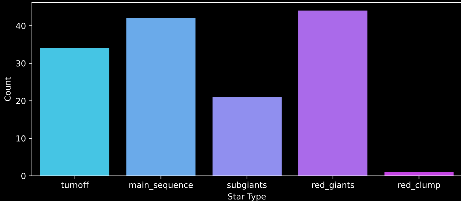
APOGEE DR17 Field: [SMC8] Count plot of Star Type
