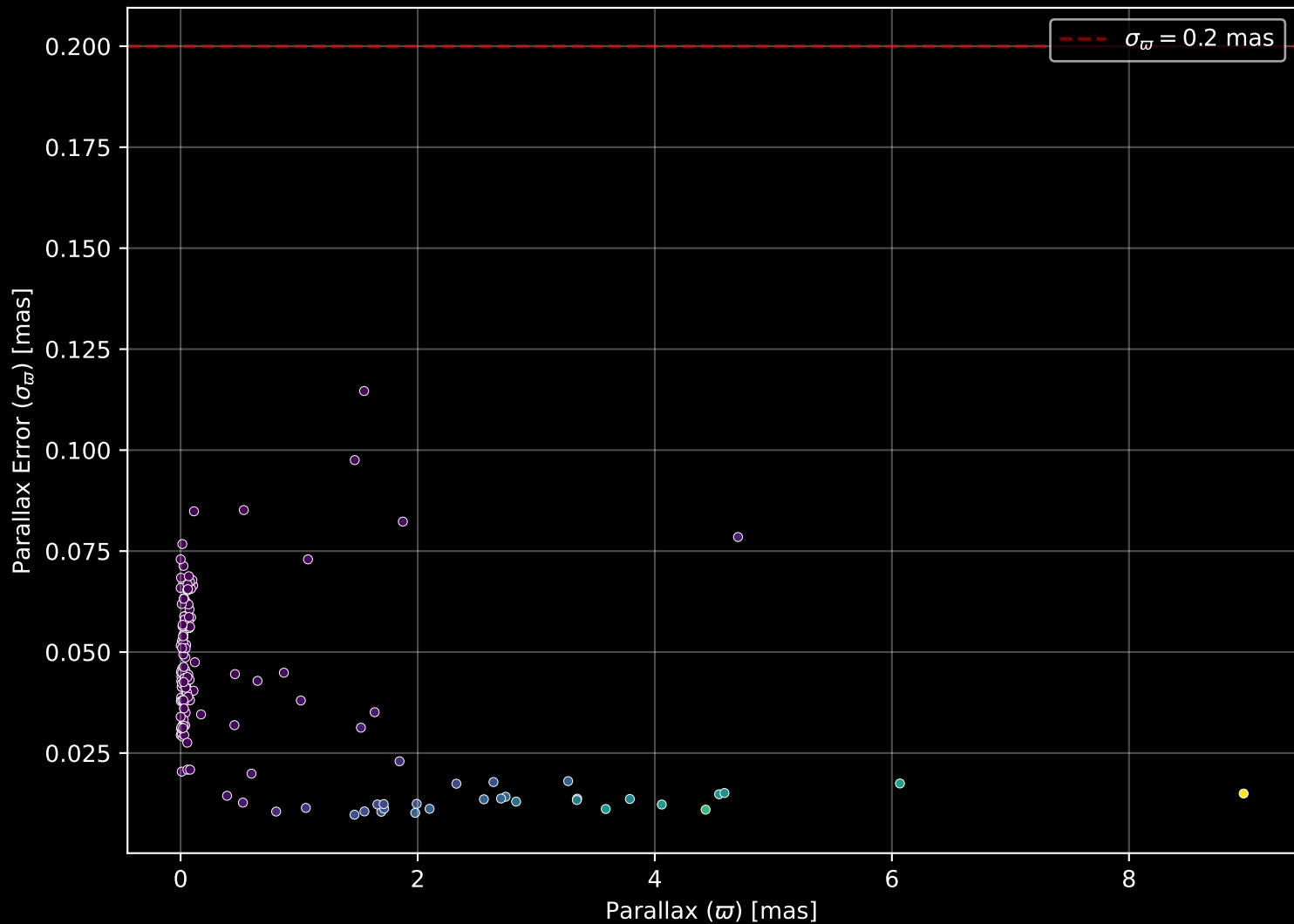
APOGEE DR17 Field: [SMC8] Parallax Quality (n= 142)
