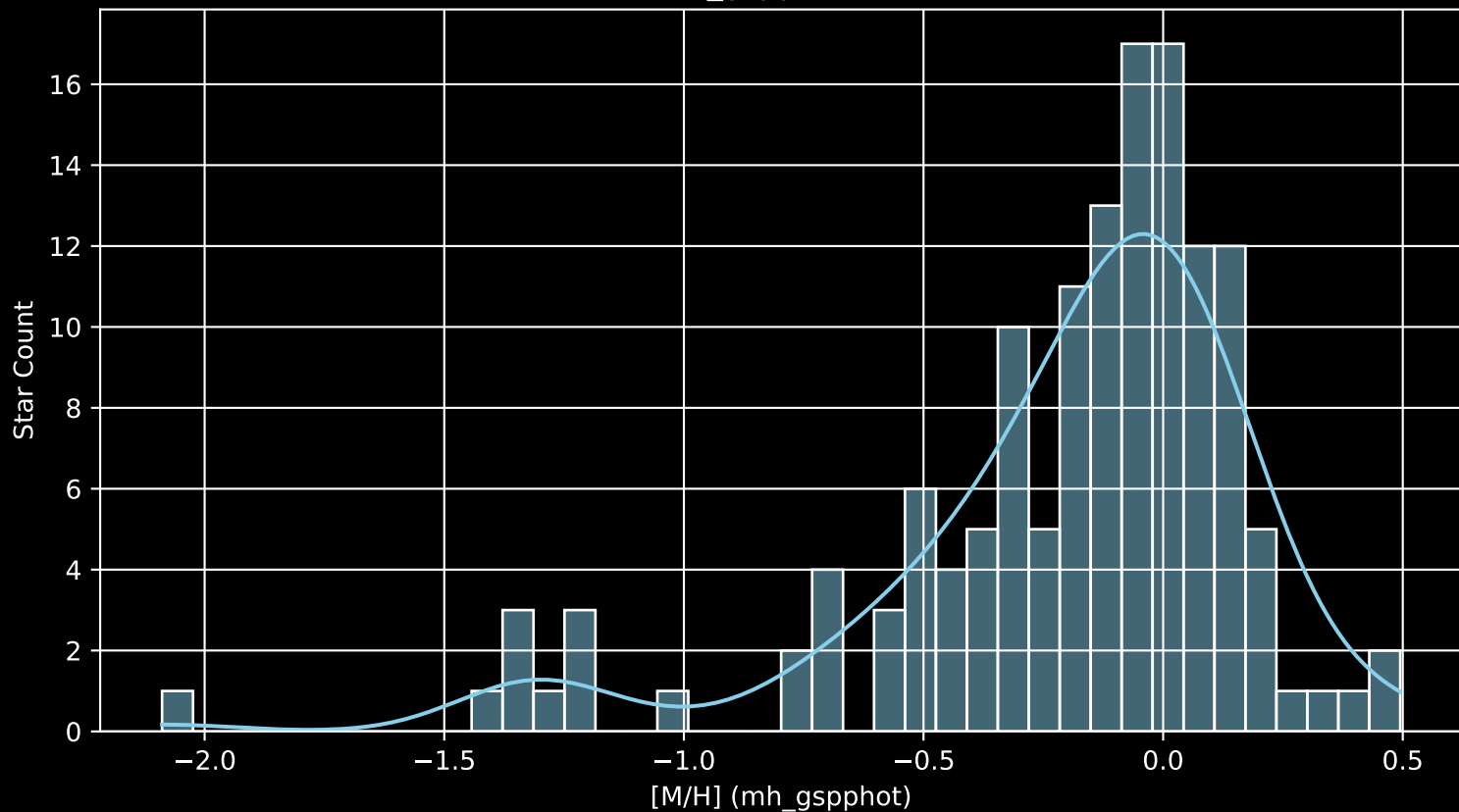
APOGEE DR17 Field: [SMC8 [M/H] (mh_gspphot) (n= 141)
